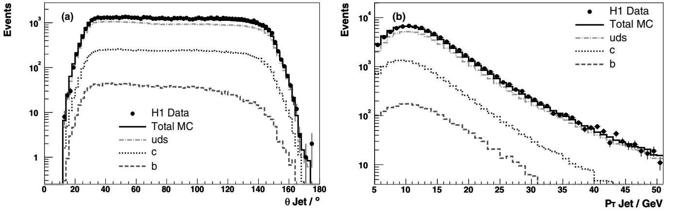
Fig. 2. The polar angle distribution a and transverse momentum distribution b of the highest p_T jet which contains at least one reconstructed CST track within a cone of radius 1. If there are no reconstructed jets the complete hadronic final state is used to define the jet axis. Included in the figure is the expectation from the RAPGAP Monte Carlo simulation showing the contributions from the various quark flavours after applying the scale factors obtained from the fit to the subtracted significance distributions of the data
