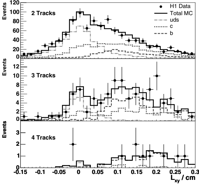
Fig. 8. The transverse distance between the primary and secondary vertex ( L_{xy} ) for events with two, three and four CST tracks associated with the secondary vertex. Superimposed on the data points are c , b and light quark contributions that have been scaled by the results of the fit to the S_1 and S_2 data distributions
