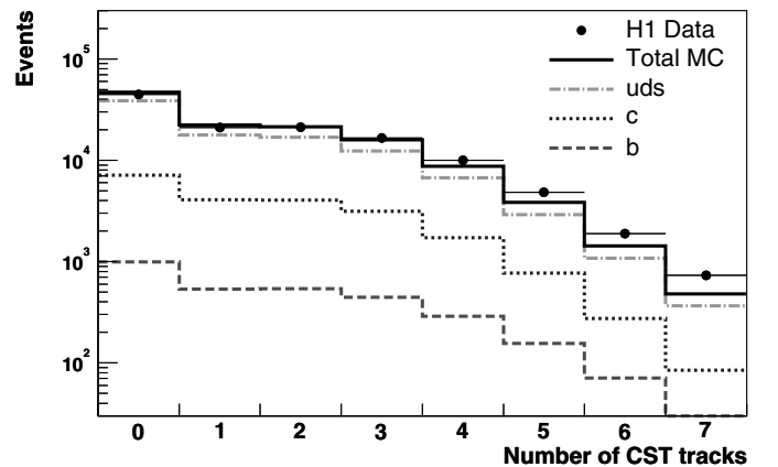
Fig. 3. The number of reconstructed central silicon tracker (CST) tracks per event associated to the jet axis. Each CST track is required to have at least two CST hits and p_T > 0.5 \text{ GeV} . Included in the figure is the expectation from the RAPGAP Monte Carlo simulation, showing the contributions from the various quark flavours after applying the scale factors obtained from the fit to the subtracted significance distributions of the data
