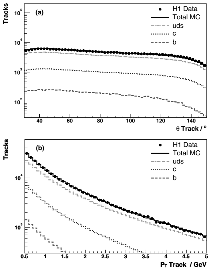
Fig. 1. The polar angle distribution a and transverse momentum distribution b of all HFS CST tracks. Included in the figure is the expectation from the RAPGAP Monte Carlo simulation, showing the contributions from the various quark flavours after applying the scale factors obtained from the fit to the subtracted significance distributions of the data (see Sect. 4.4)
