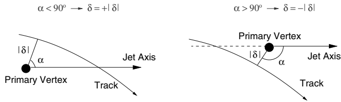
Fig. 4. Schematic diagram explaining the definition of the signed impact parameter \delta . It is defined as positive if the angle \alpha between the jet axis and the line joining the primary vertex to the point of DCA is less than 90^\circ , and is defined as negative otherwise
