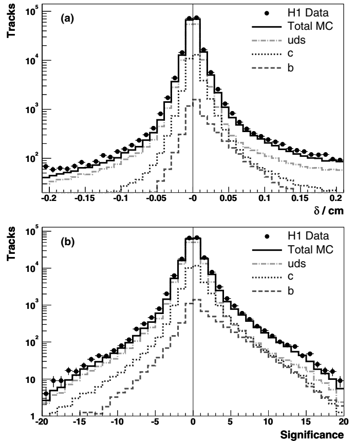
Fig. 5. The signed impact parameter \delta of a track to the primary vertex in the x - y plane a and the significance \delta/\sigma(\delta) b , where \sigma(\delta) is the error on \delta , for all CST tracks associated to the jet axis. The cut |\delta| < 0.1 cm has been applied in figure b . Included in the figure is the expectation from the RAPGAP Monte Carlo simulation, showing the contributions from the various quark flavours after applying the scale factors obtained from the fit to the subtracted significance distributions of the data
