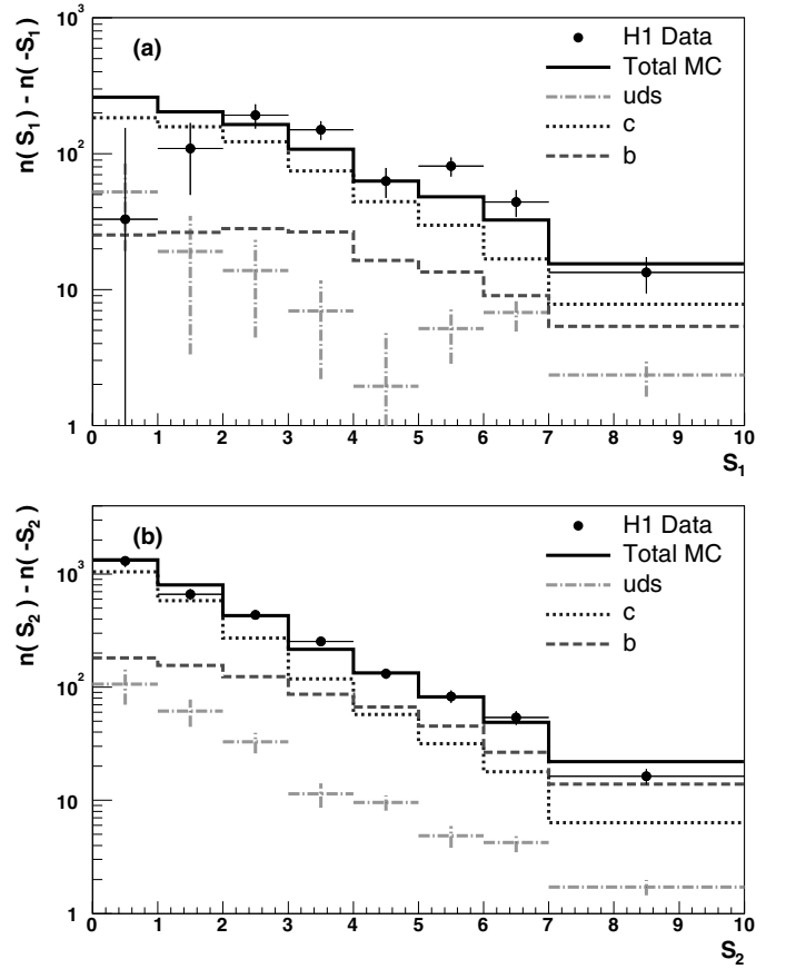
Fig. 7. The subtracted distributions of a S_1 and b S_2 . Included in the figure is the result from the fit to the data of the Monte Carlo distributions of the various quark flavours
