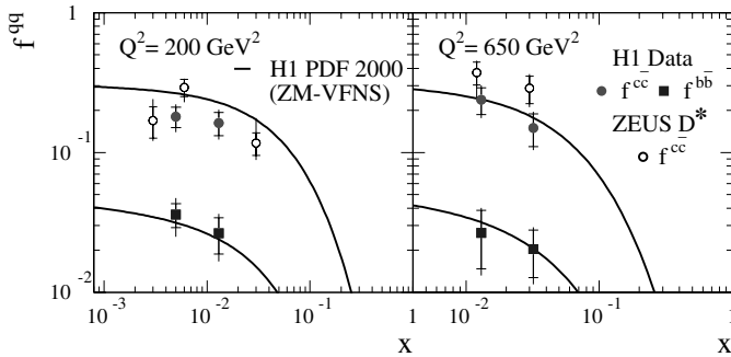
Fig. 10. The contributions to the total cross section f^{c\bar{c}} and f^{b\bar{b}} shown as a function of x for two different Q^2 values. The inner error bars show the statistical error, the outer error bars represent the statistical and systematic errors added in quadrature. The f^{c\bar{c}} from ZEUS obtained from measurements of D^* mesons [2] and the prediction of the H1 NLO QCD fit [16] are also shown
